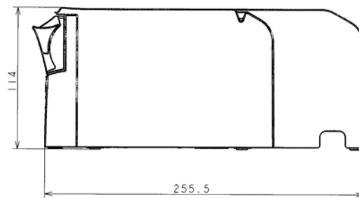
Figure 5-26 When the optional OT-CC70 is installed
