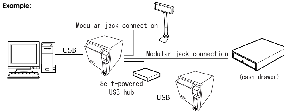
Figure 2-17 USB connection
