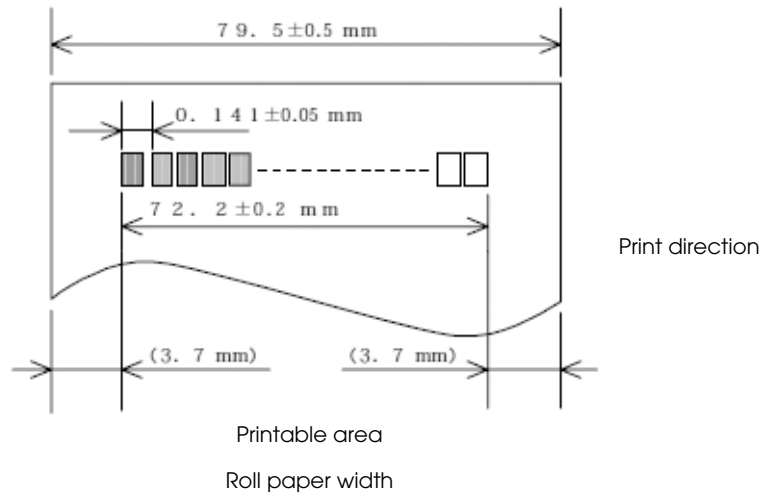
Figure 5-23 Printable area
