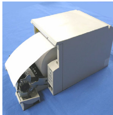
Figure 1-4 Loading paper
