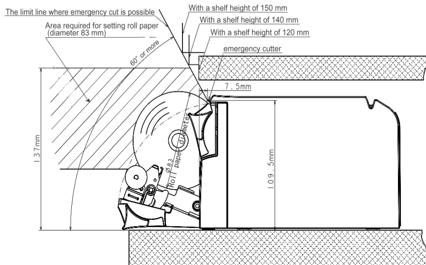
Figure 2-10 Placed on a shelf
