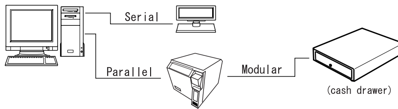
Figure 2-16 Parallel interface connection
