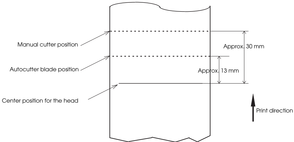
Figure 5-24 Print position versus cutter position
