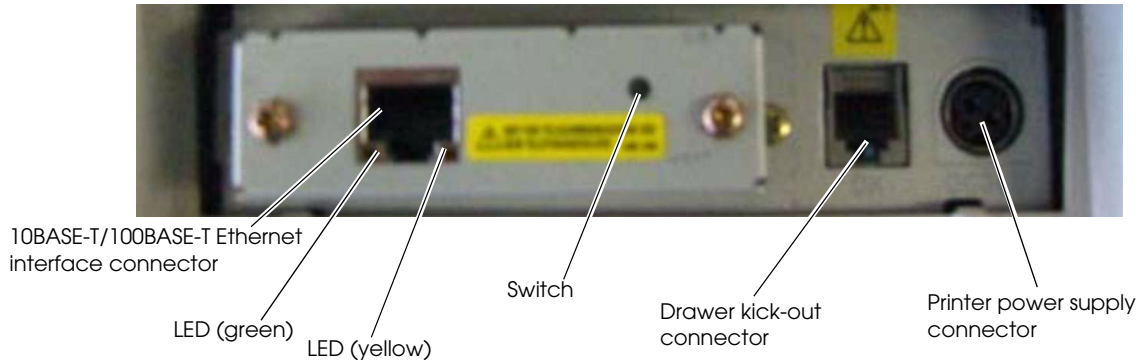
Figure 2-20 Example Ethernet port interface panel (UB-E02)
