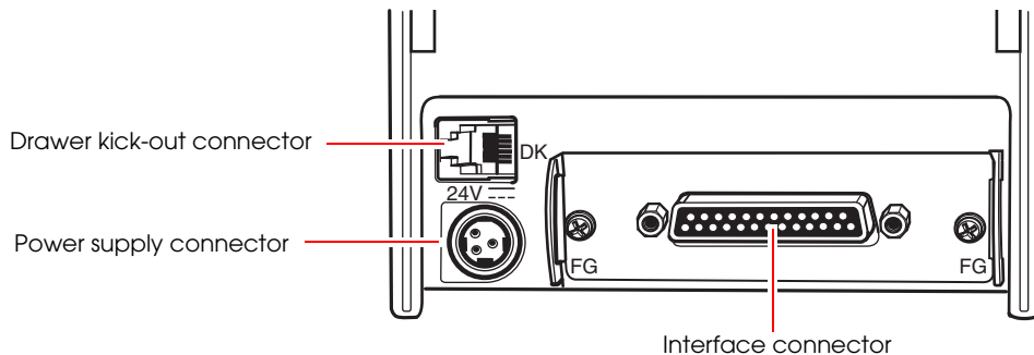
Figure 2-15 Printer connectors
