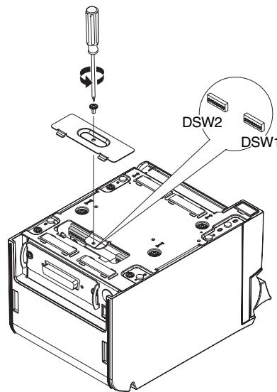
Figure 2-11 Removing the DIP switch cover
