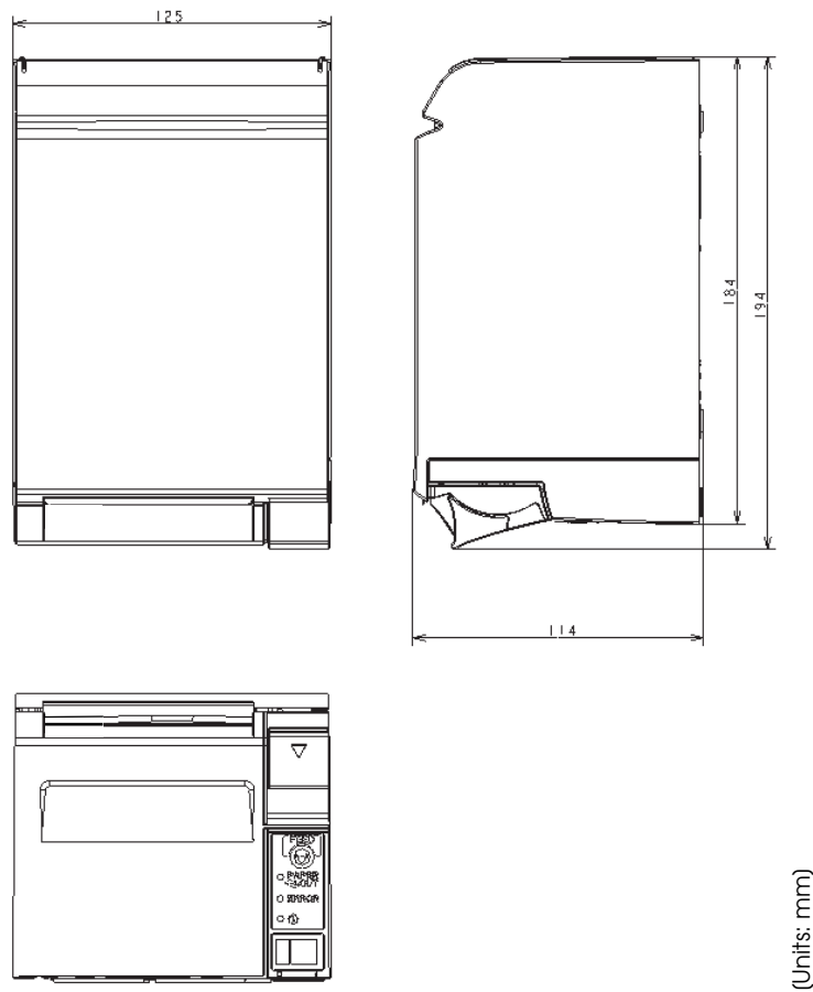
Figure 5-25 Dimensions
