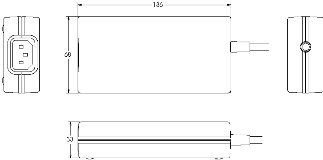
Figure B-1 Case specifications
