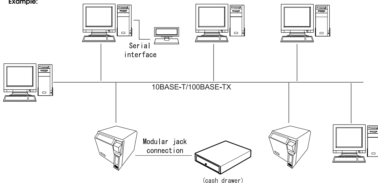
Figure 2-19 Ethernet connection
