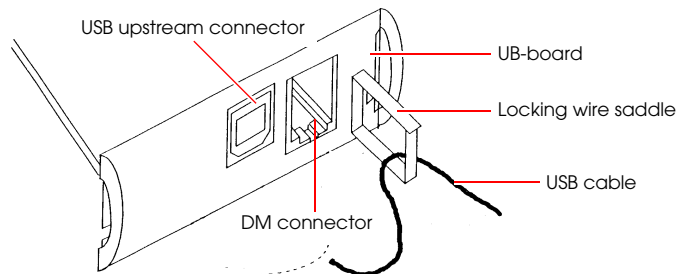
Figure 2-18 Installing the locking wire saddle
