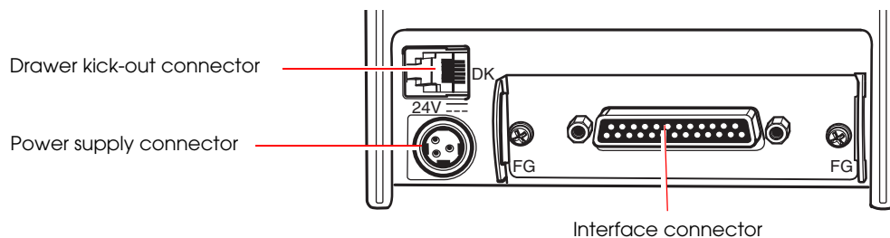
Figure 1-2 Connector panel
